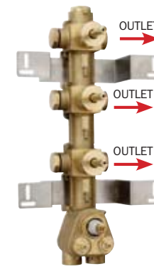
THERMOSTATIC Z030202000 3 OUTLETS
